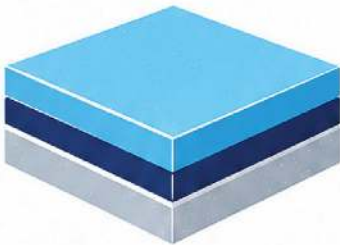
Epoxy
